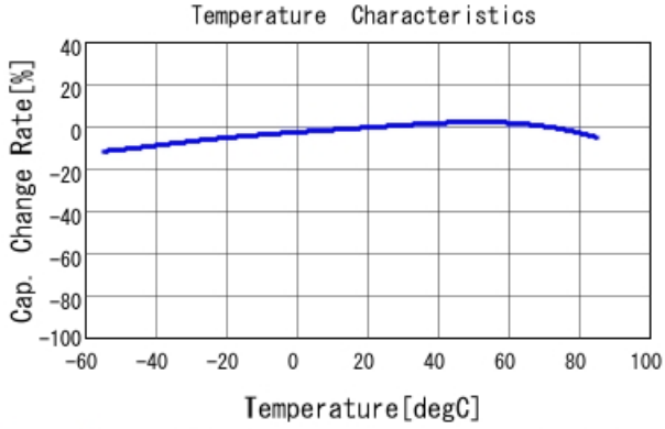
GRM188R61H474KA12 C-Temp. capchange, DC0.0V, AC1.5
