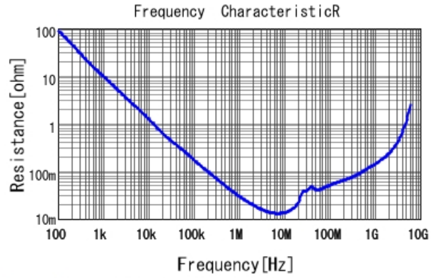
GRM188R61H474KA12 R DCOV, 25degC
