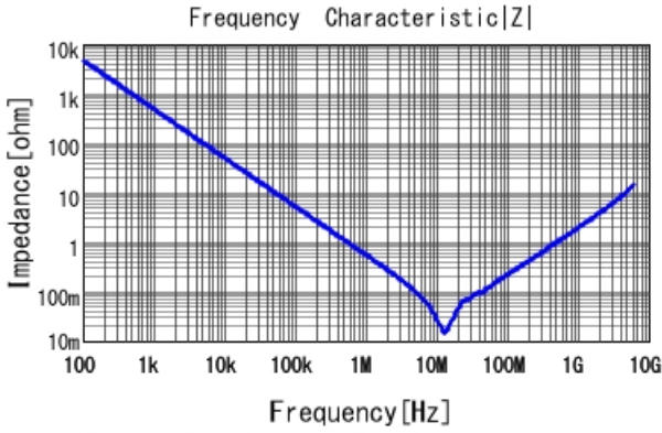
GRM188R61H474KA12 |Z| DCOV, 25degC
