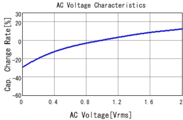
GRM188R61H474KA12 C-AC Voltage capchange, DCOV, 25
