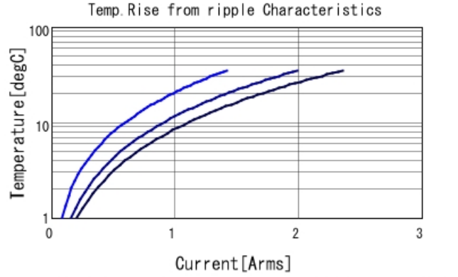
GRM188R61H474KA12 Temp. rise — 200kHz — 500
