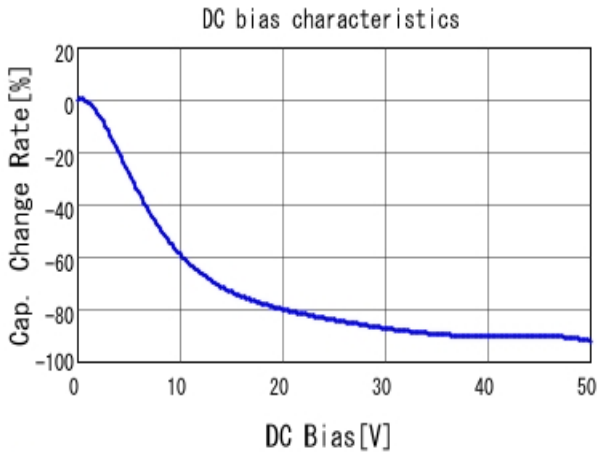
■ GRM188R61H225KE11 C-DC bias capchange, 25.0degC, AC1V
