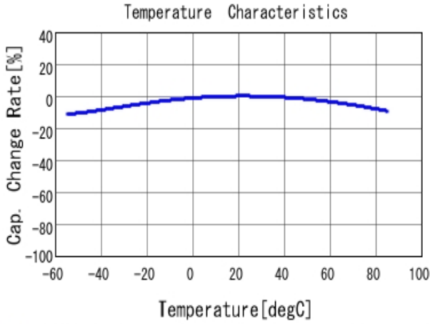
■ GRM188R61H225KE11 C-Temp. capchange, DCO. 0V, ACO. 5V rm
