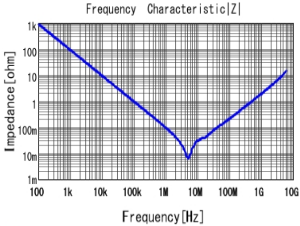
■ GRM188R61H225KE11 |Z| DCOV, 25degC
