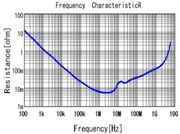
■ GRM188R61H225KE11 R DCOV, 25degC
