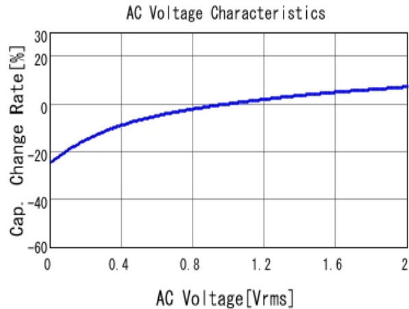
■ GRM188R61H225KE11 C-AC Voltage capchange, DCOV, 25.0d
