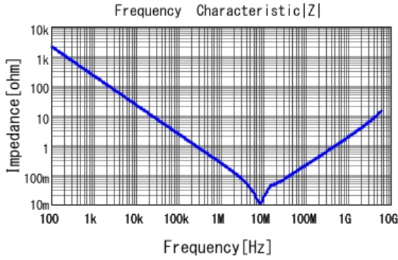
■ GRM188R61H105KAAL |Z| DCOV, 25degC
