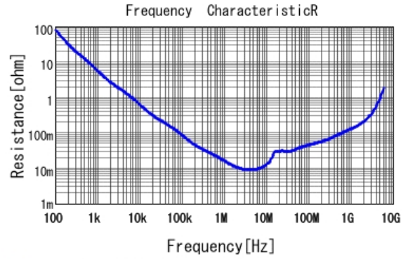
■ GRM188R61H105KAAL R DCOV, 25degC
