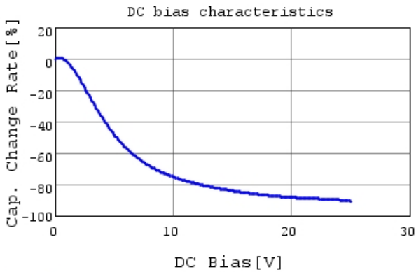
GRM188R61E475KE11 C-DC bias capchange, 25.0c
