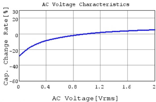
GRM188R61E475KE11 C-AC Voltage capchange, Dc
