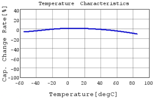
GRM188R61E475KE11 C-Temp. capchange, DCO.0V,
