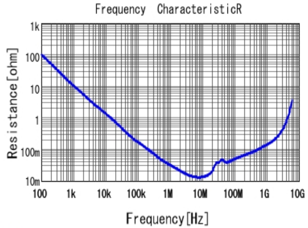
■ GRM188R61E474KA12 R DCOV, 25degC
