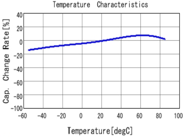
■ GRM188R61E474KA12 C-Temp. capchange, DCO. 0V, AC1.0V r m
