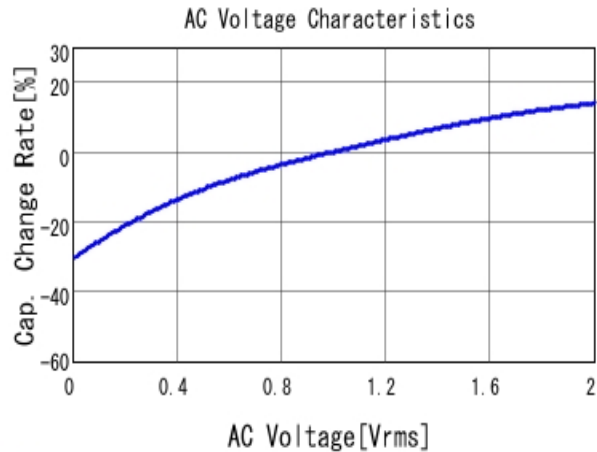
■ GRM188R61E474KA12 C-AC Voltage capchange, DCOV, 25.0d
