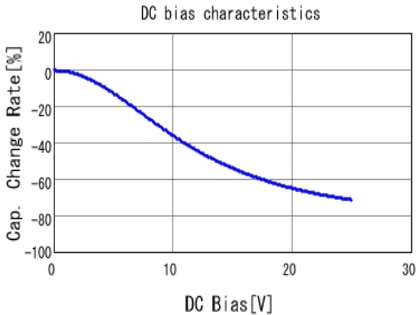
■ GRM188R61E474KA12 C-DC bias capchange, 25.0degC, AC1.
