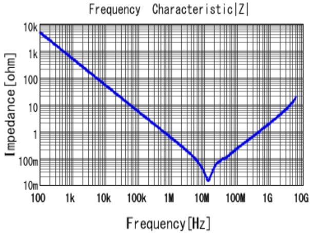
■ GRM188R61E474KA12 |Z| DCOV, 25degC
