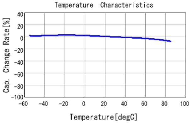
■ GRM188R61E225MA12 C-Temp. capchange, DCO. 0V, AC1. 0Vrm
