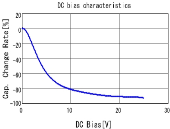
■ GRM188R61E106MA73 C-DC bias capchange, 25.0degC, AC1V
