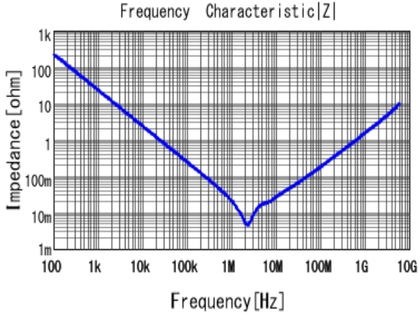
■ GRM188R61E106MA73 |Z| DCOV, 25degC
