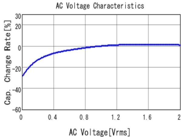
■ GRM188R61E106MA73 C-AC Voltage capchange, DCOV, 25.0d
