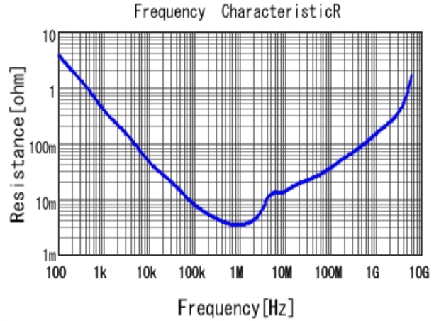
■ GRM188R61E106MA73 R DCOV, 25degC
