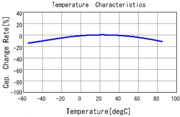
GRM188R61E106MA73 C-Temp. capchange, DC0.0V, ACO.2
