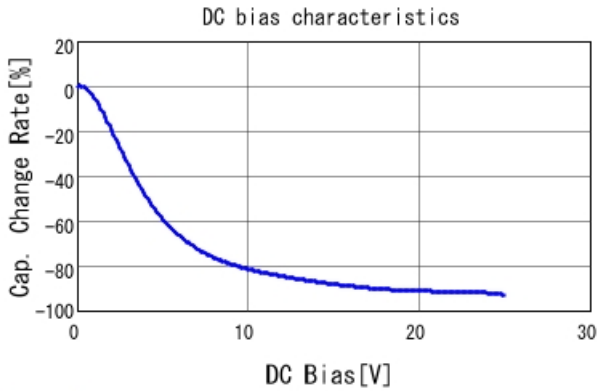
GRM188R61E106MA73 C-DC bias capchange, 25.0degC, A
