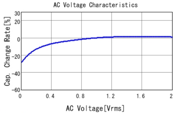
GRM188R61E106MA73 C-AC Voltage capchange, DCOV, 25
