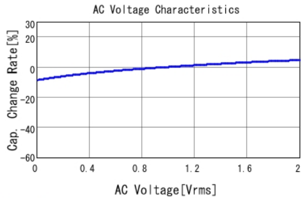
GRM188R61E105KAAD C-AC Voltage capchange, DCOV, 25
