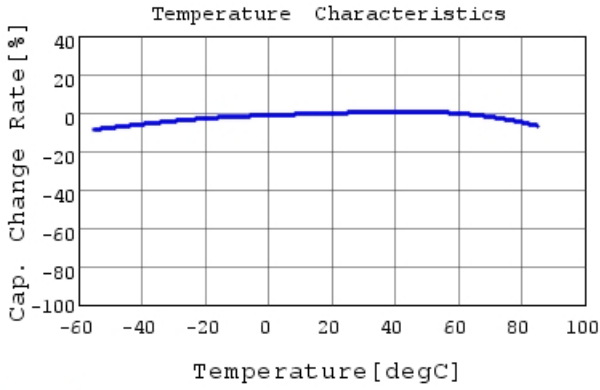
GRM188R61E105KA12 C-Temp. capchange, DC0.0V,
