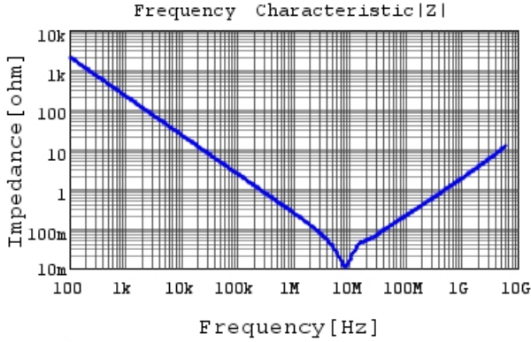
GRM188R61E105KA12 |Z| DCOV, 25degC
