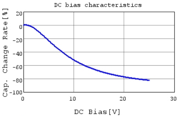
GRM188R61E105KA12 C-DC bias capchange, 25.0c
