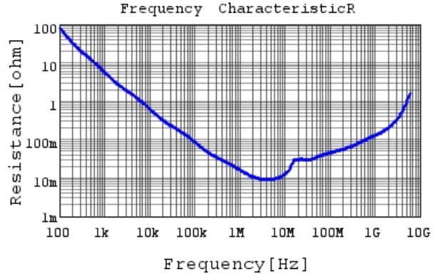
GRM188R61E105KA12 R DCOV, 25degC
