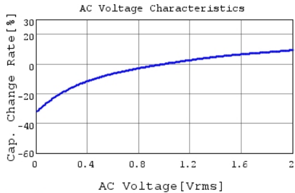
GRM188R61E105KA12 C-AC Voltage capchange, DC
