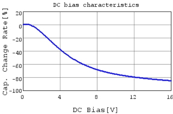
GRM188R61C475KE11 C-DC bias capchange, 25.0c
