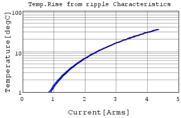
GRM188R61C475KE11 Temp.rise 500kHz
