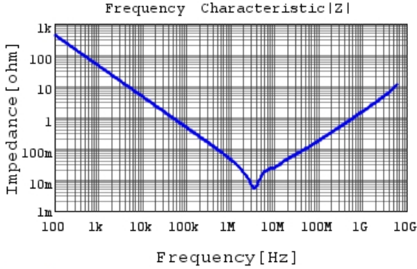
GRM188R61C475KE11 |Z| DCOV,25degC
