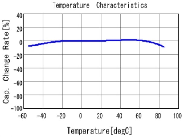
■ GRM188R61C225KE15 C-Temp. capchange, DC0.0V, AC0.5V rm
