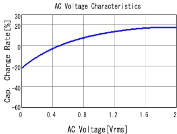
■ GRM188R61C225KE15 C-AC Voltage capchange, DCOV, 25.0d
