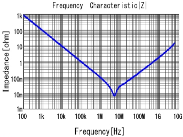
■ GRM188R61C225KE15 |Z| DCOV, 25degC
