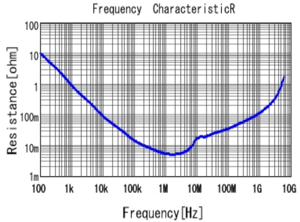
■ GRM188R61C225KE15 R DCOV, 25degC
