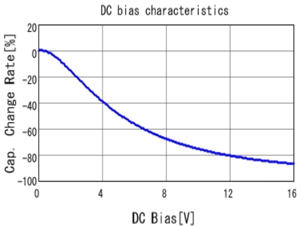
■ GRM188R61C225KE15 C-DC bias capchange, 25.0degC, AC0.
