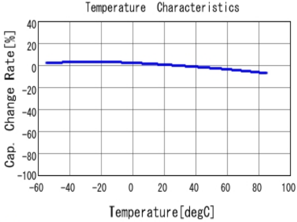
■ GRM188R61A684KA61 C-Temp. capchange, DC0.0V, AC1.0V rm
