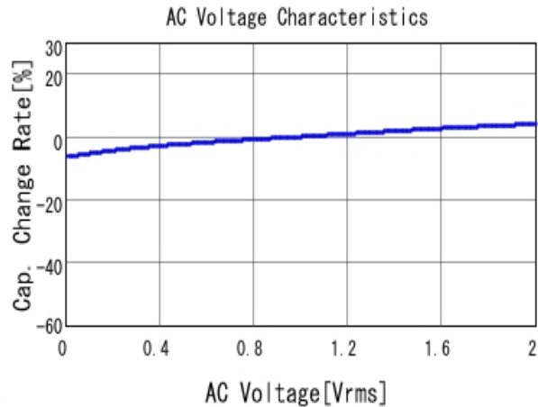
■ GRM188R61A684KA61 C-AC Voltage capchange, DCOV, 25.0d
