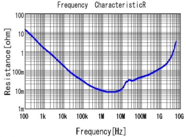
■ GRM188R61A684KA61 R DCOV, 25degC
