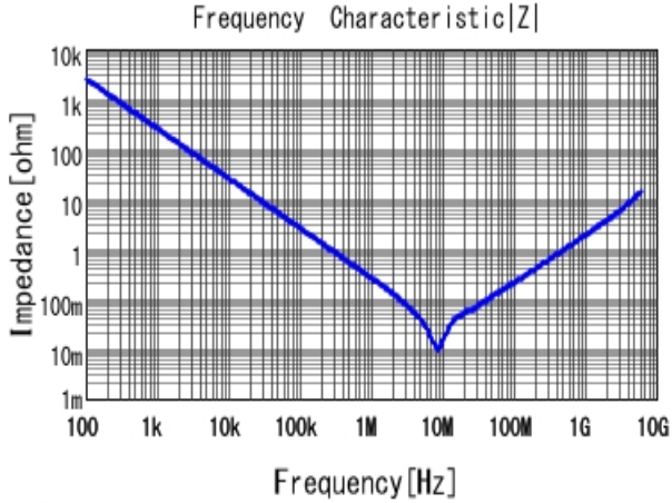
■ GRM188R61A684KA61 |Z| DCOV, 25degC
