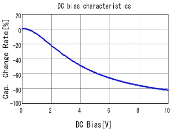
■ GRM188R61A475KE15 C-DC bias capchange, 25.0degC, AC0.
