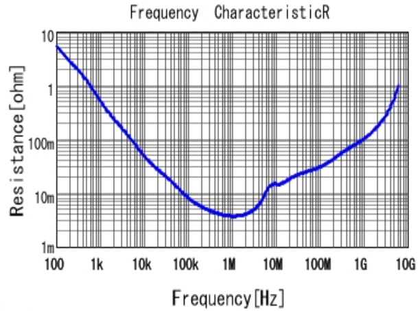
■ GRM188R61A475KE15 R DCOV, 25degC
