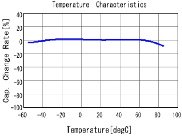
■ GRM188R61A475KE15 C-Temp. capchange, DCO. 0V, ACO. 5V rm
