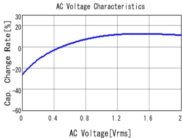
■ GRM188R61A475KE15 C-AC Voltage capchange, DCOV, 25.0d
