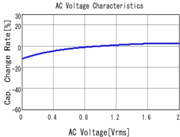
■ GRM188R61A475KAAJ C-AC Voltage capchange, DCOV, 25.0d
