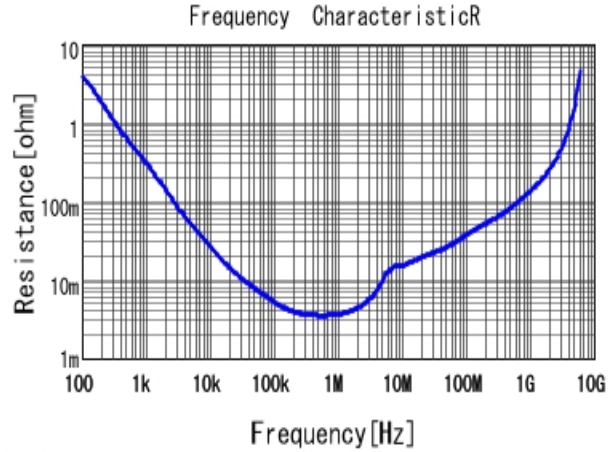
■ GRM188R61A475KAAJ R DCOV, 25degC
