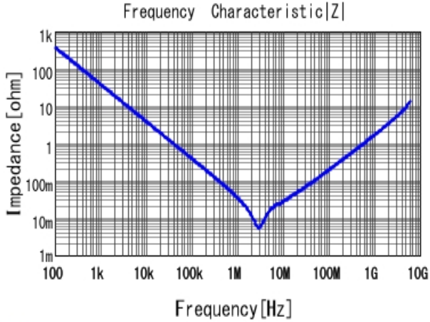
■ GRM188R61A475KAAJ |Z| DCOV, 25degC
