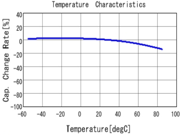
■ GRM188R61A475KAAJ C-Temp. capchange, DC0.0V, AC1.0V rm
