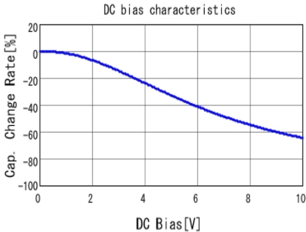
■ GRM188R61A475KAAJ C-DC bias capchange, 25.0degC, AC1.
