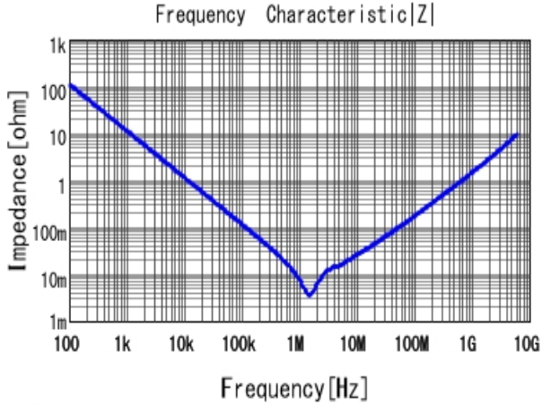
■ GRM188R61A226ME15 |Z| DCOV, 25degC
