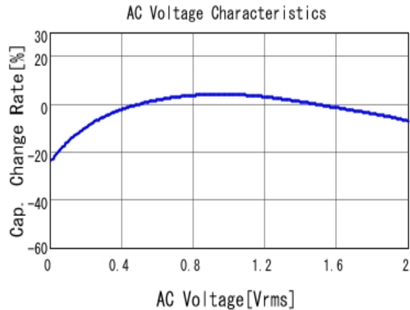
■ GRM188R61A226ME15 C-AC Voltage capchange, DCOV, 25.0d
