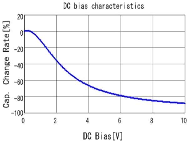
■ GRM188R61A226ME15 C-DC bias capchange, 25.0degC, AC0.
