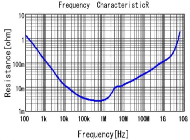
■ GRM188R61A226ME15 R DCOV, 25degC
