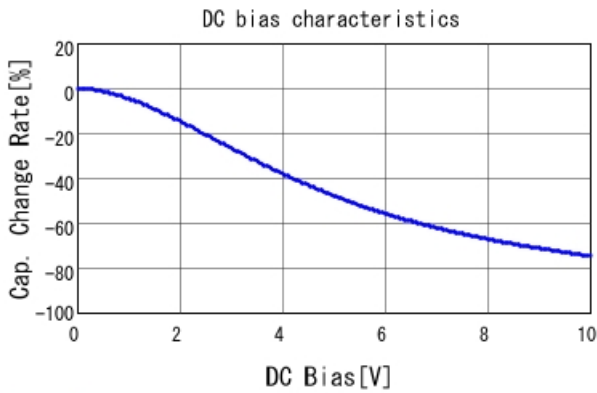
GRM188R61A225KE34 C-DC bias capchange, 25.0degC, A
