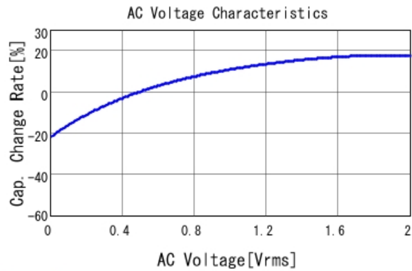
GRM188R61A225KE34 C-AC Voltage capchange, DCOV, 25
