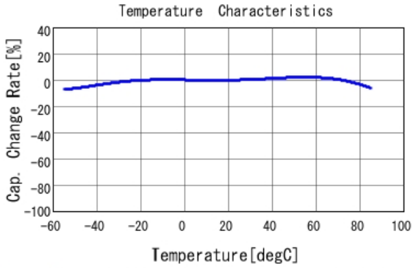
GRM188R61A225KE34 C-Temp. capchange, DC0.0V, ACO.5
