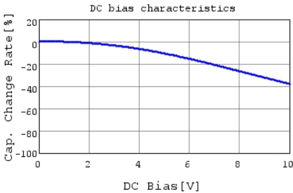
GRM188R61A105KA61 C-DC bias capchange, 25.0c
