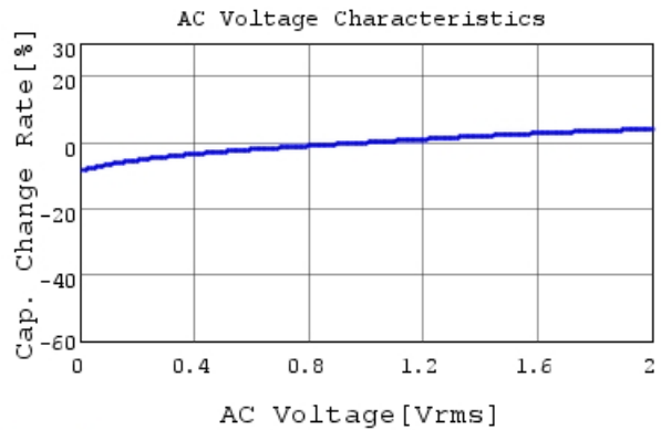
GRM188R61A105KA61 C-AC Voltage capchange, DC
