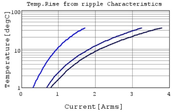
GRM188R61A105KA61 Temp.rise — 100kHz
