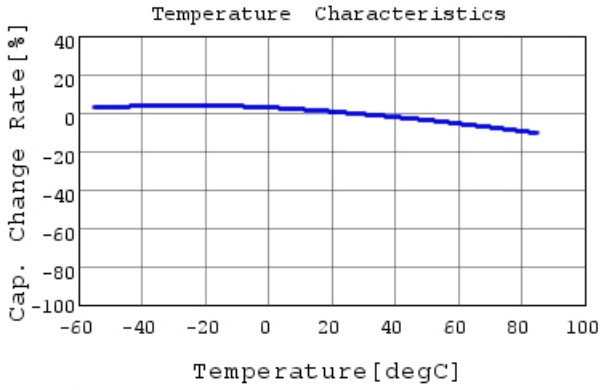
GRM188R61A105KA61 C-Temp. capchange, DCO.0V,
