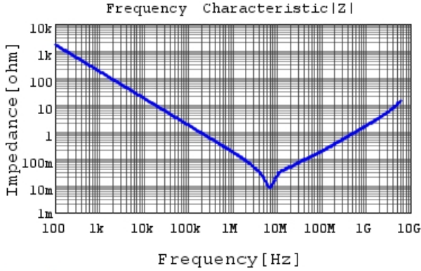
GRM188R61A105KA61 |Z| DCOV, 25degC
