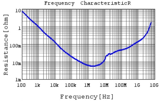
GRM188R61A105KA61 R DCOV, 25degC
