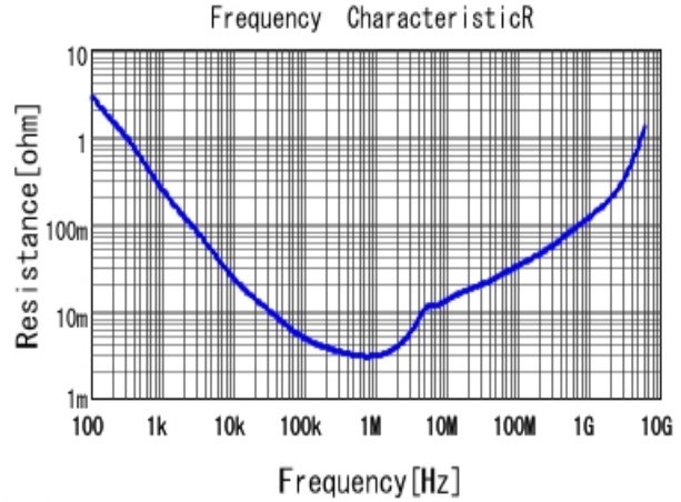
■ GRM188R60J106ME47 R DCOV, 25degC
