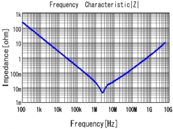
■ GRM188R60J106ME47 |Z| DCOV, 25degC
