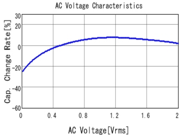
■ GRM188R60J106ME47 C-AC Voltage capchange, DCOV, 25.0d
