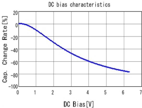
■ GRM188R60J106ME47 C-DC bias capchange, 25.0degC, AC0.
