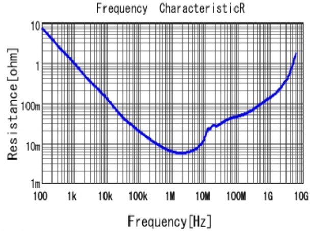
■ GRM188R60J105KA01 R DCOV, 25degC
