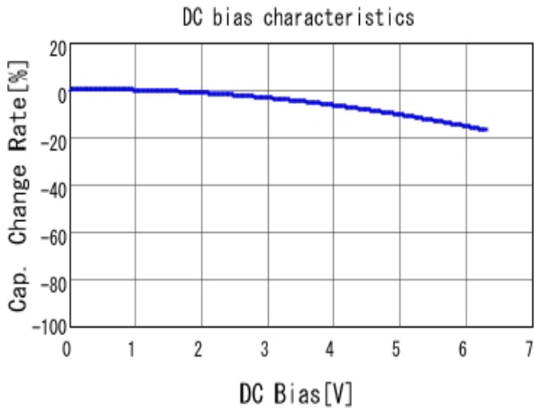
■ GRM188R60J105KA01 C-DC bias capchange, 25.0degC, AC1.
