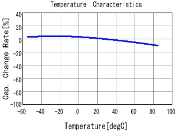
■ GRM188R60J105KA01 C-Temp. capchange, DC0.0V, AC1.0V r m
