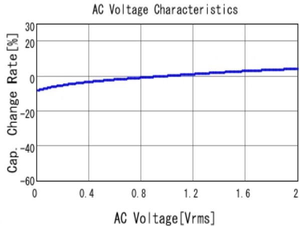
■ GRM188R60J105KA01 C-AC Voltage capchange, DCOV, 25.0d
