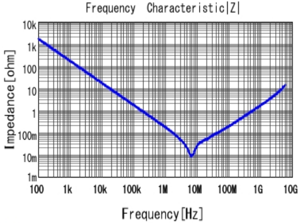
■ GRM188R60J105KA01 |Z| DCOV, 25degC
