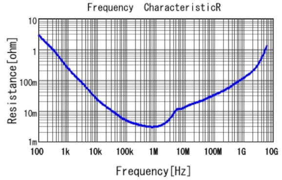
■ GRM188R60G106ME47 R DCOV, 25degC
