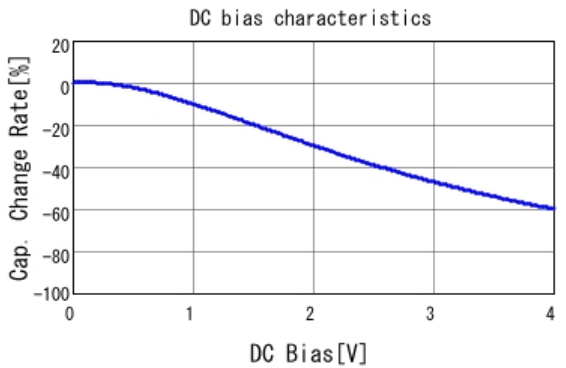
■ GRM188R60G106ME47 C-DC bias capchange, 25.0degC, AC0.
