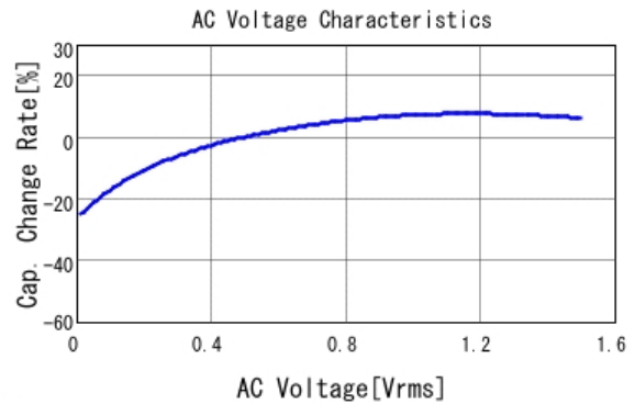
■ GRM188R60G106ME47 C-AC Voltage capchange, DCOV, 25.0d
