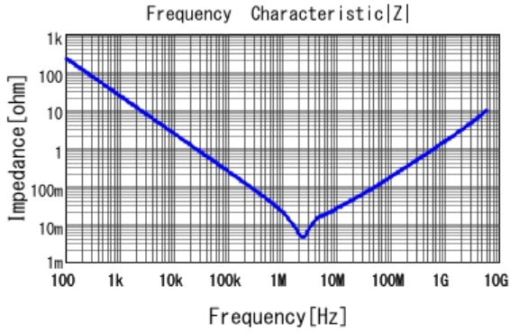
■ GRM188R60G106ME47 |Z| DCOV, 25degC
