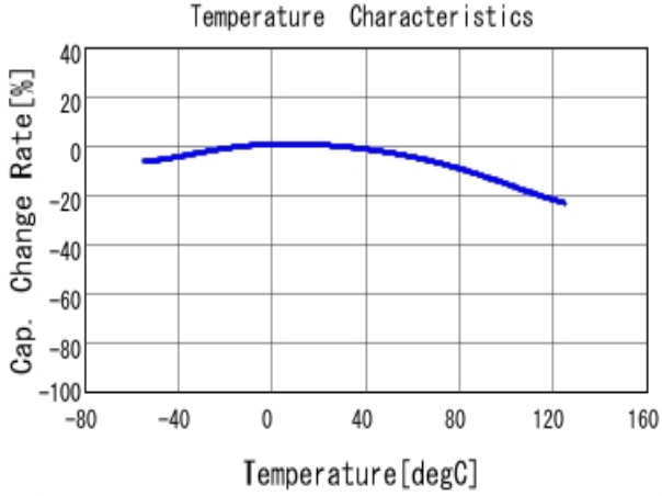
■ GRM188D71A475KE11 C-Temp. capchange, DCO. 0V, ACO. 5V rm
