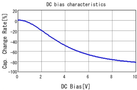
■ GRM188D71A106MA73 C-DC bias capchange, 25.0degC, AC1V
