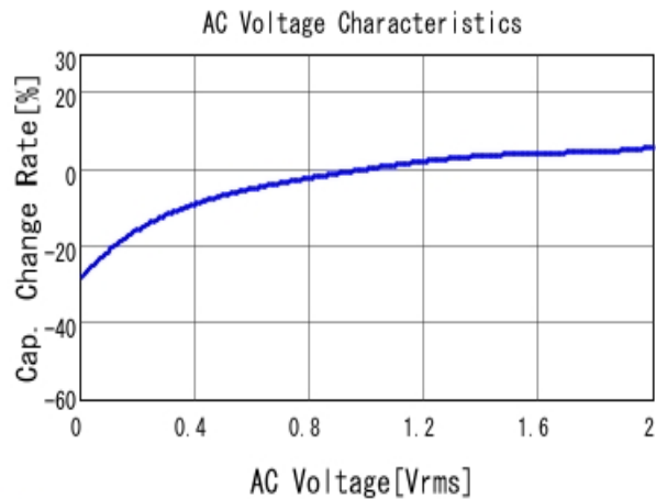
■ GRM188C81E475KE11 C-AC Voltage capchange, DCOV, 25.0d
