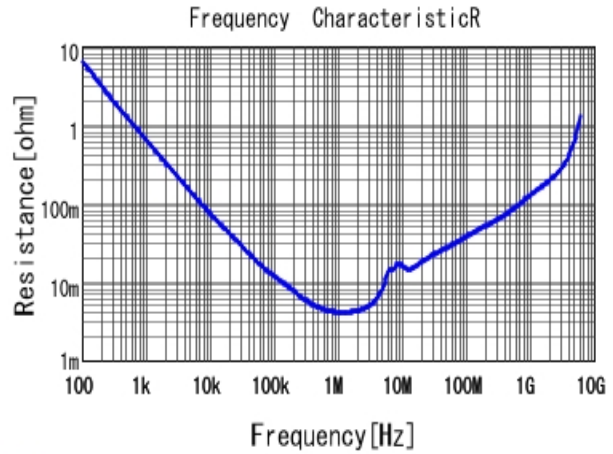
■ GRM188C81E475KE11 R DCOV, 25degC
