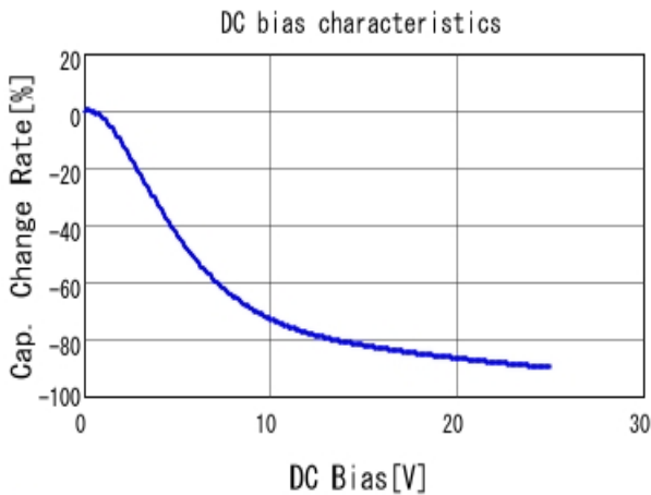
■ GRM188C81E475KE11 C-DC bias capchange, 25.0degC, AC1V
