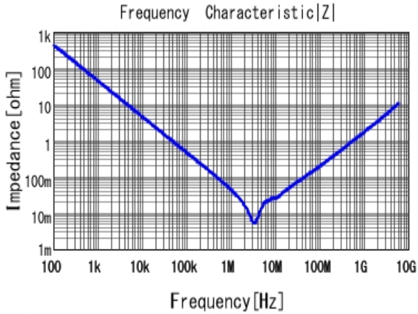
■ GRM188C81E475KE11 |Z| DCOV, 25degC
