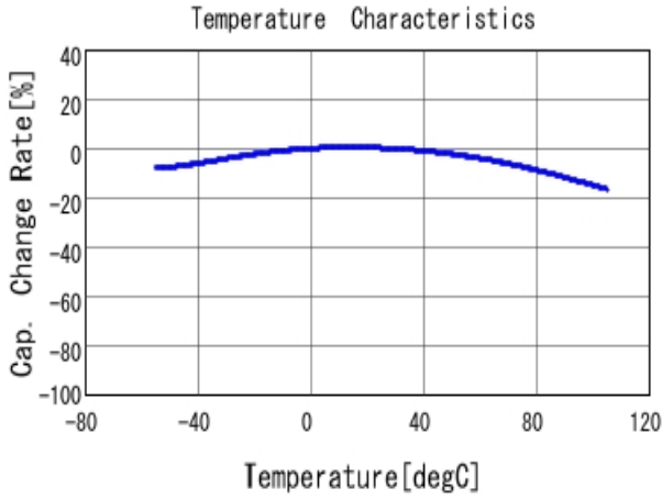
■ GRM188C81E475KE11 C-Temp. capchange, DCO. 0V, ACO. 5V rm
