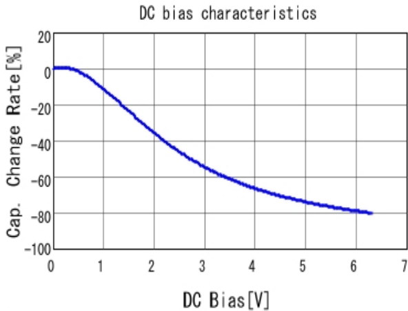
■ GRM188C80J226ME15 C-DC bias capchange, 25.0degC, AC0.
