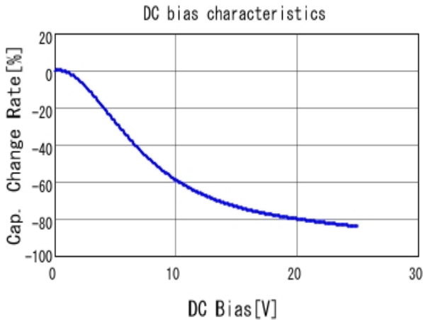
■ GRM188C71E225KE11 C-DC bias capchange, 25.0degC, AC1V
