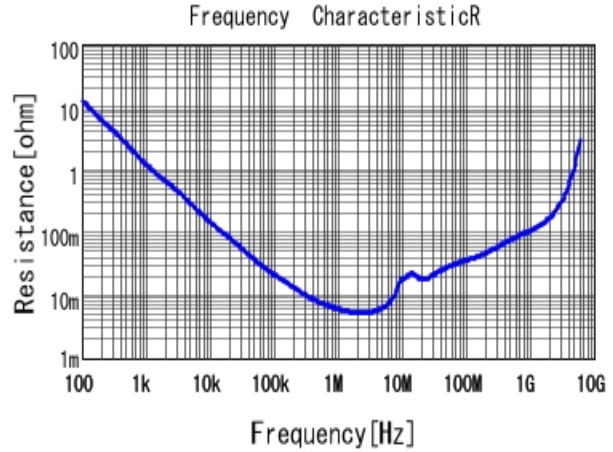
■ GRM188C71E225KE11 R DCOV, 25degC
