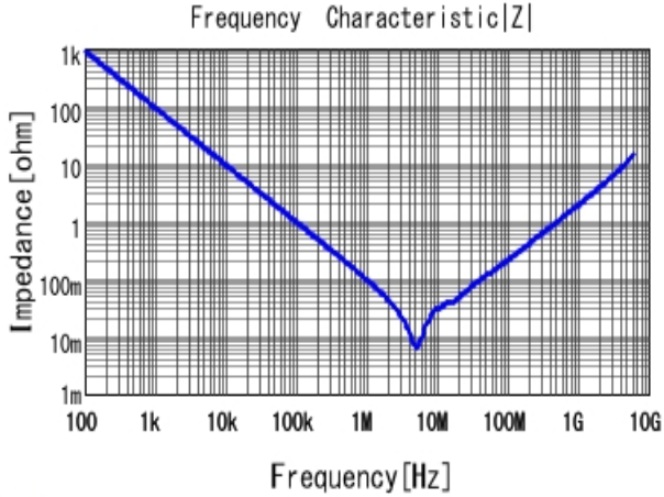
■ GRM188C71E225KE11 |Z| DCOV, 25degC
