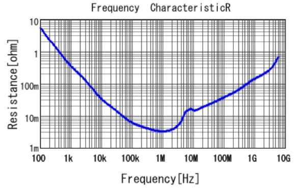
■ GRM188C71C475KE21 R DCOV, 25degC
