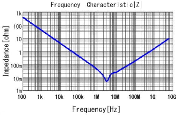
■ GRM188C71C475KE21 |Z| DCOV, 25degC
