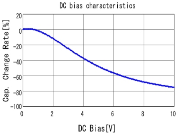
■ GRM188C71A475KE11 C-DC bias capchange, 25.0degC, AC1V
