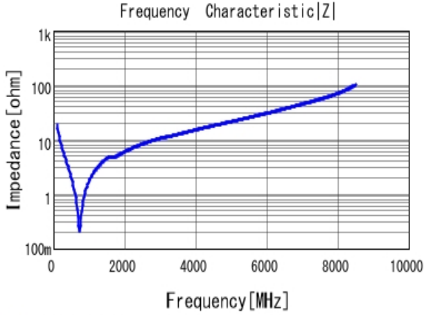
■ GRM1885C2A820JA01 |Z| DCOV, 25degC
