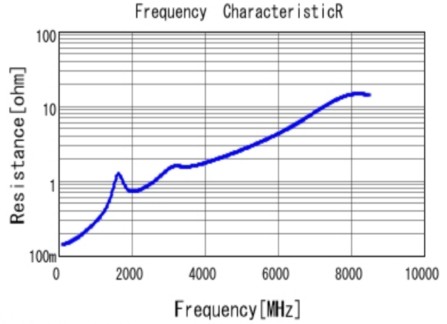
■ GRM1885C2A820JA01 R DCOV, 25degC
