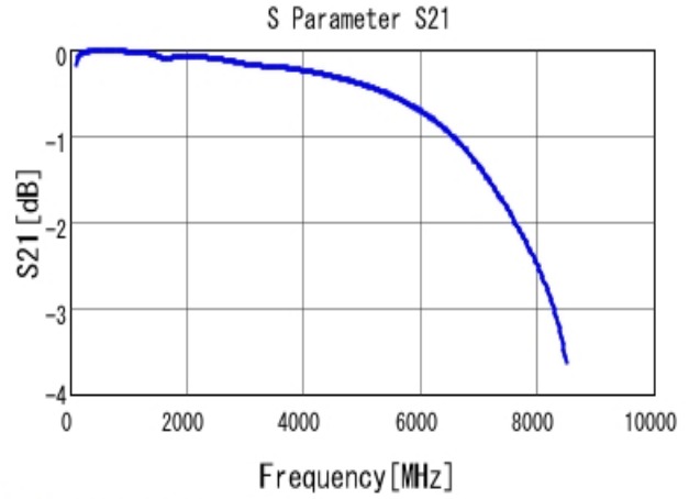
■ GRM1885C2A820JA01 S21 DCOV, 25degC
