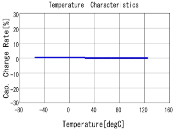
■ GRM1885C2A820JA01 C-Temp. capchange, DCOV, AC1Vrms
