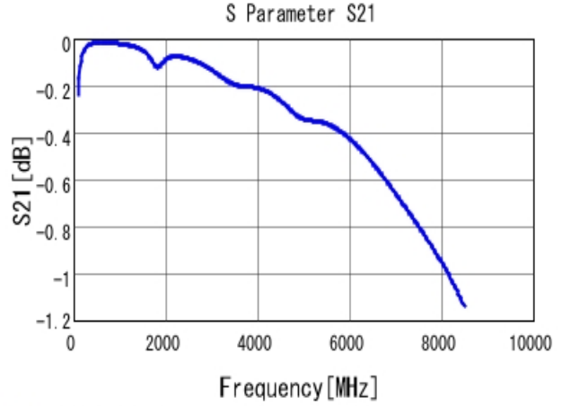
■ GRM1885C2A680JA01 S21 DCOV, 25degC
