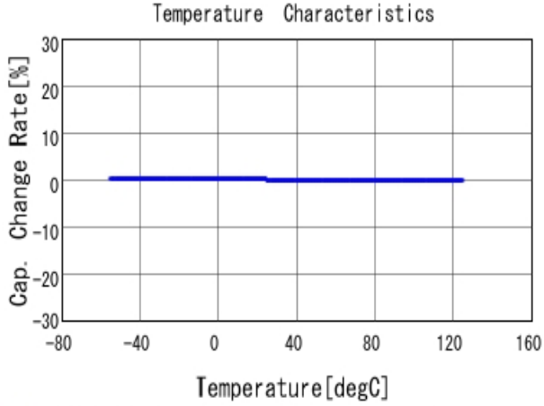
■ GRM1885C2A680JA01 C-Temp. capchange, DCOV, AC1Vrms
