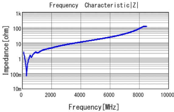
■ GRM1885C2A561JA01 |Z| DCOV, 25degC
