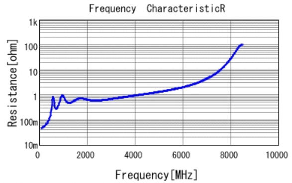
■ GRM1885C2A561JA01 R DCOV, 25degC
