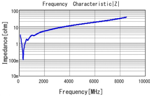
■ GRM1885C2A471JA01 |Z| DCOV, 25degC
