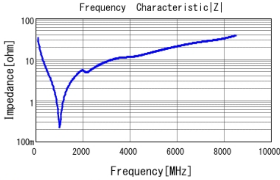
■ GRM1885C2A470JA01 |Z| DCOV, 25degC
