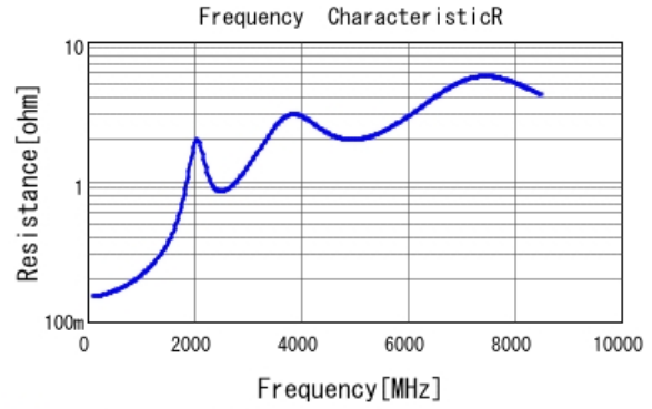
■ GRM1885C2A470JA01 R DCOV, 25degC
