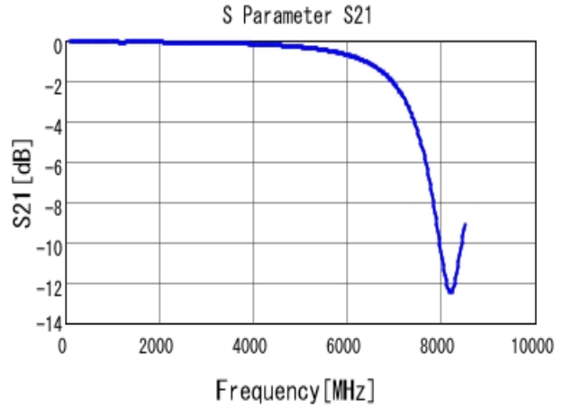
■ GRM1885C2A391JA01 S21 DCOV, 25degC
