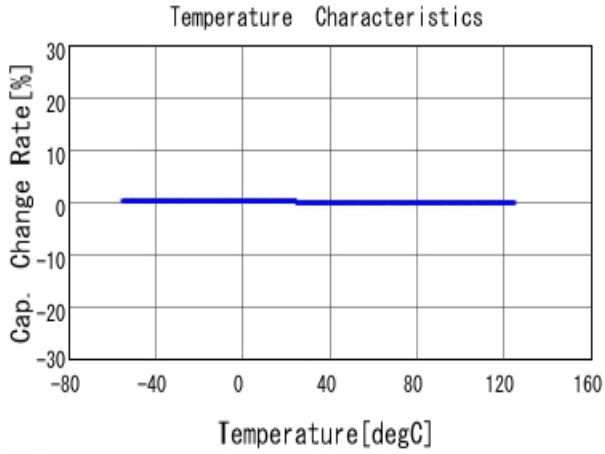
■ GRM1885C2A391JA01 C-Temp. capchange, DCOV, AC1Vrms
