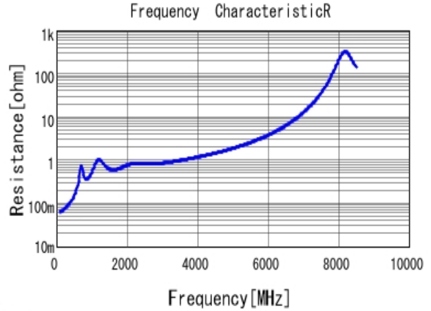
■ GRM1885C2A391JA01 R DCOV, 25degC
