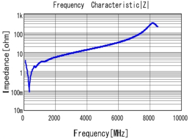
■ GRM1885C2A391JA01 |Z| DCOV, 25degC
