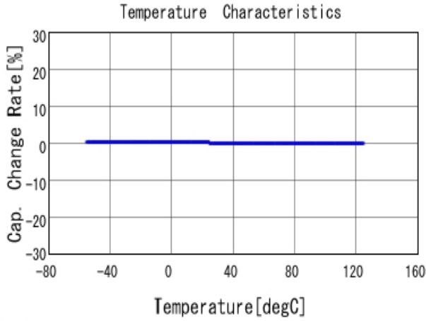
■ GRM1885C2A390JA01 C-Temp. capchange, DCOV, AC1Vrms
