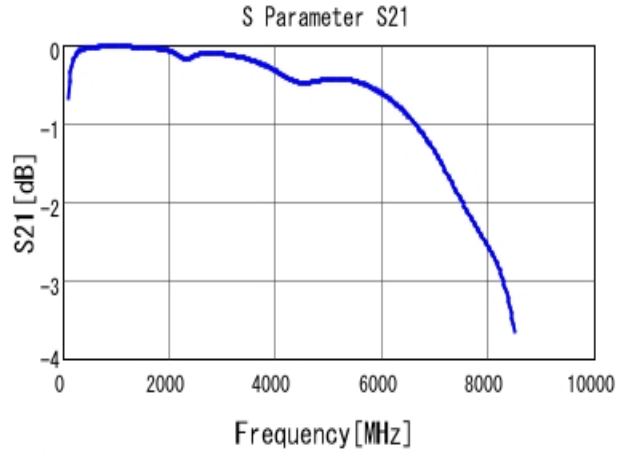
■ GRM1885C2A390JA01 S21 DCOV, 25degC
