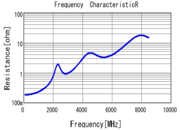
■ GRM1885C2A390JA01 R DCOV, 25degC
