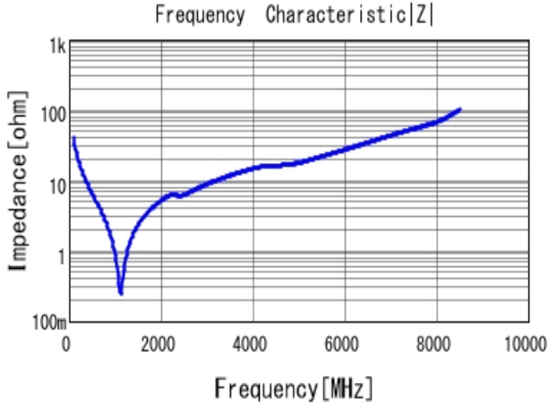
■ GRM1885C2A390JA01 |Z| DCOV, 25degC
