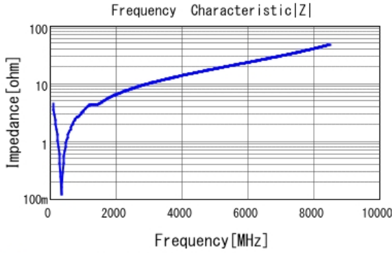
■ GRM1885C2A331JA01 |Z| DCOV, 25degC
