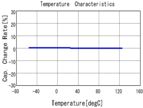
■ GRM1885C2A330JA01 C-Temp. capchange, DCOV, AC1Vrms
