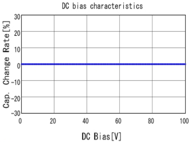
■ GRM1885C2A330JA01 C-DC bias capchange, 25.0degC, AC1V
