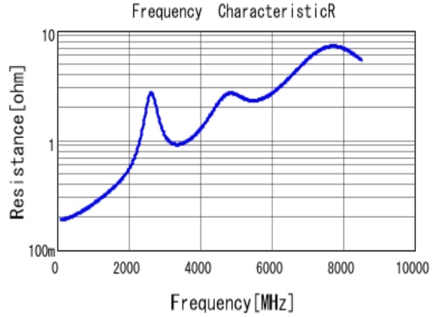
■ GRM1885C2A330JA01 R DCOV, 25degC
