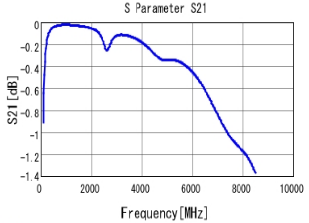
■ GRM1885C2A330JA01 S21 DCOV, 25degC
