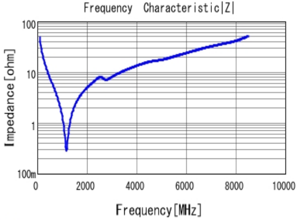
■ GRM1885C2A330JA01 |Z| DCOV, 25degC
