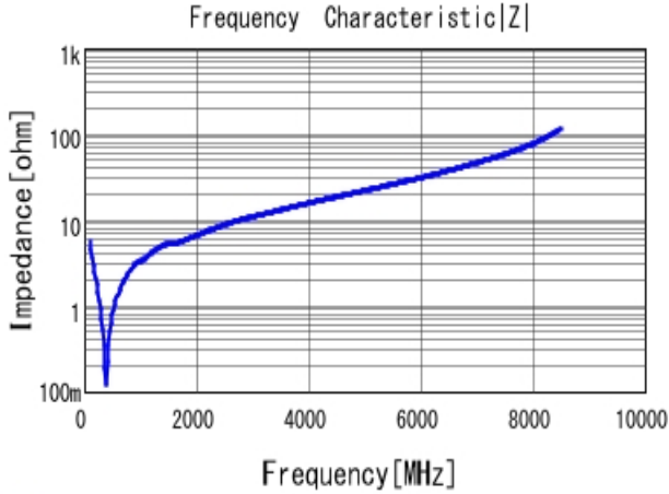
■ GRM1885C2A271JA01 |Z| DCOV, 25degC
