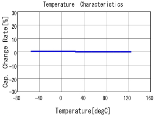
■ GRM1885C2A271JA01 C-Temp. capchange, DCOV, AC1Vrms
