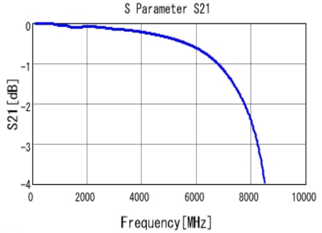
■ GRM1885C2A271JA01 S21 DCOV, 25degC
