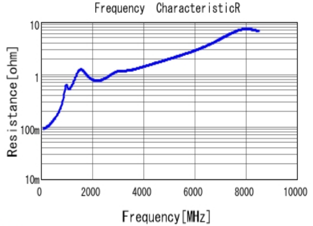
■ GRM1885C2A271JA01 R DCOV, 25degC
