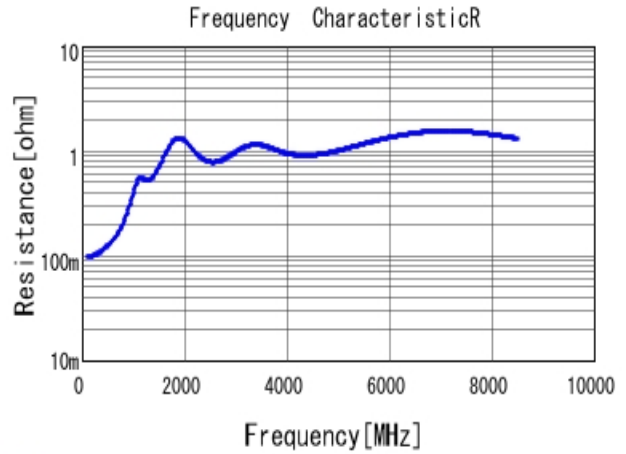
■ GRM1885C2A221JA01 R DCOV, 25degC
