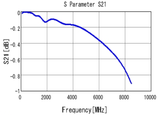
■ GRM1885C2A221JA01 S21 DCOV, 25degC
