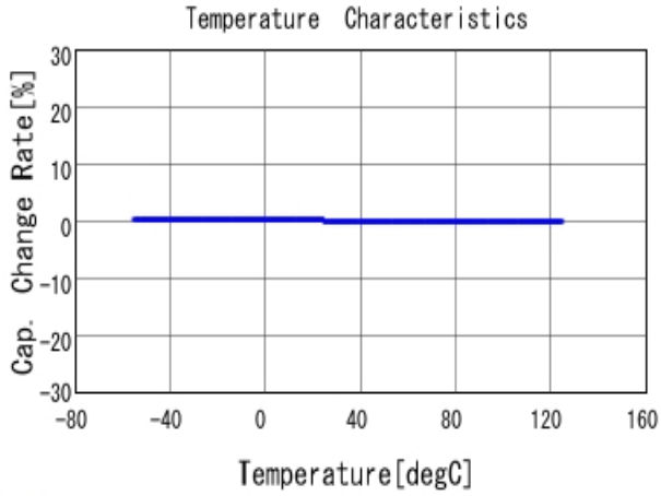
■ GRM1885C2A221JA01 C-Temp. capchange, DCOV, AC1Vrms
