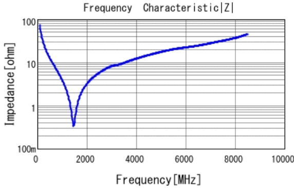
■ GRM1885C2A220JA01 |Z| DCOV, 25degC
