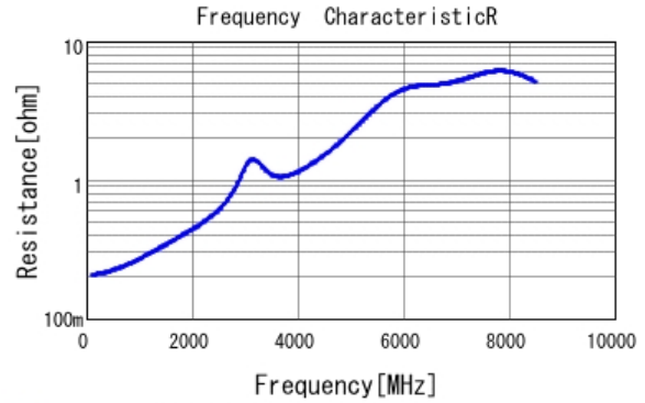
■ GRM1885C2A220JA01 R DCOV, 25degC
