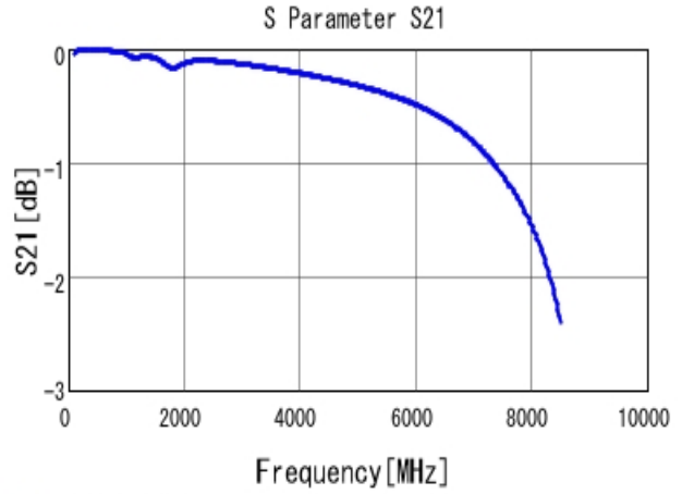
■ GRM1885C2A181JA01 S21 DCOV, 25degC
