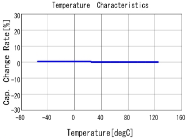
■ GRM1885C2A181JA01 C-Temp. capchange, DCOV, AC1Vrms
