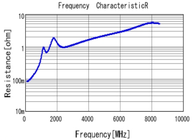
■ GRM1885C2A181JA01 R DCOV, 25degC
