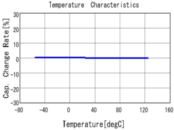
■ GRM1885C2A180JA01 C-Temp. capchange, DCOV, AC1Vrms
