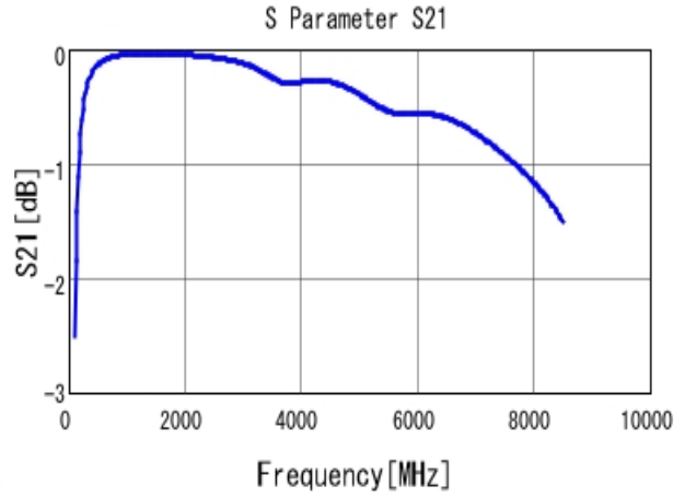
■ GRM1885C2A180JA01 S21 DCOV, 25degC
