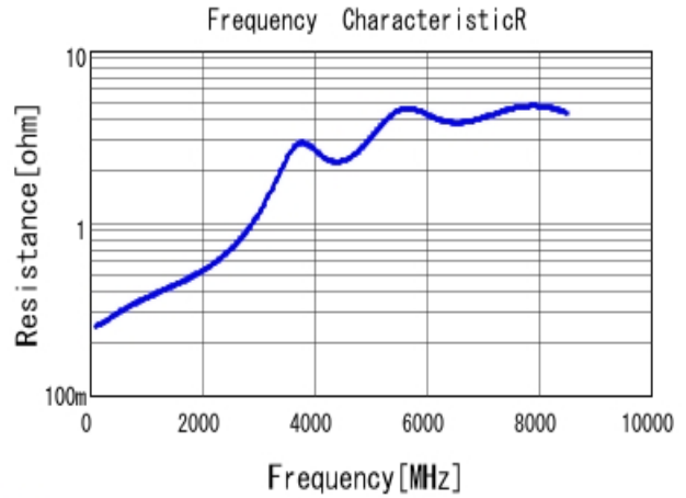
■ GRM1885C2A180JA01 R DCOV, 25degC
