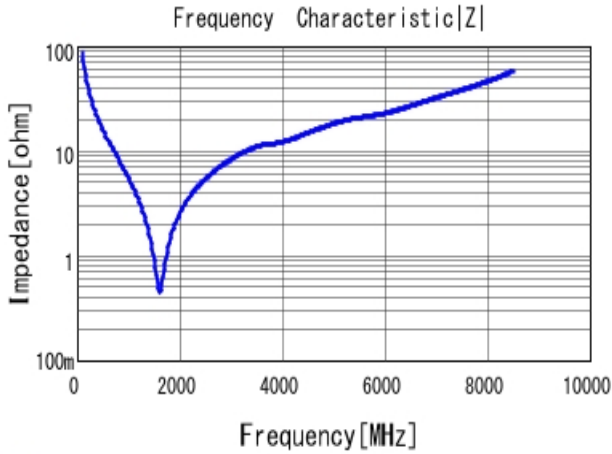
■ GRM1885C2A180JA01 |Z| DCOV, 25degC
