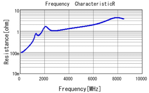
■ GRM1885C2A151JA01 R DCOV, 25degC
