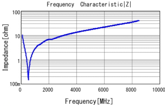
■ GRM1885C2A151JA01 |Z| DCOV, 25degC
