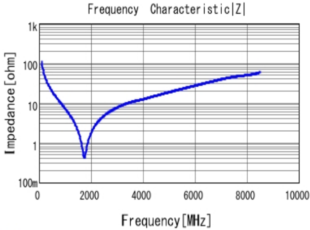
■ GRM1885C2A150JA01 |Z| DCOV, 25degC
