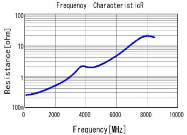
■ GRM1885C2A150JA01 R DCOV, 25degC
