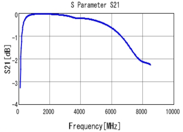
■ GRM1885C2A150JA01 S21 DCOV, 25degC
