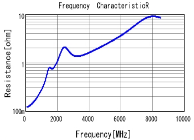
■ GRM1885C2A121JA01 R DCOV, 25degC
