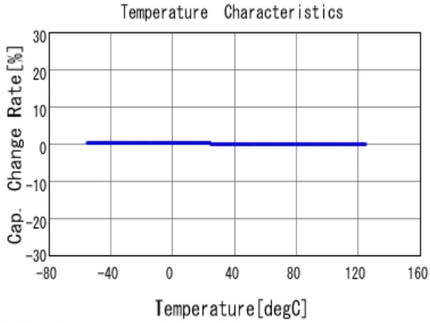
■ GRM1885C2A121JA01 C-Temp. capchange, DCOV, AC1Vrms
