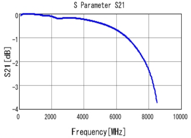
■ GRM1885C2A121JA01 S21 DCOV, 25degC
