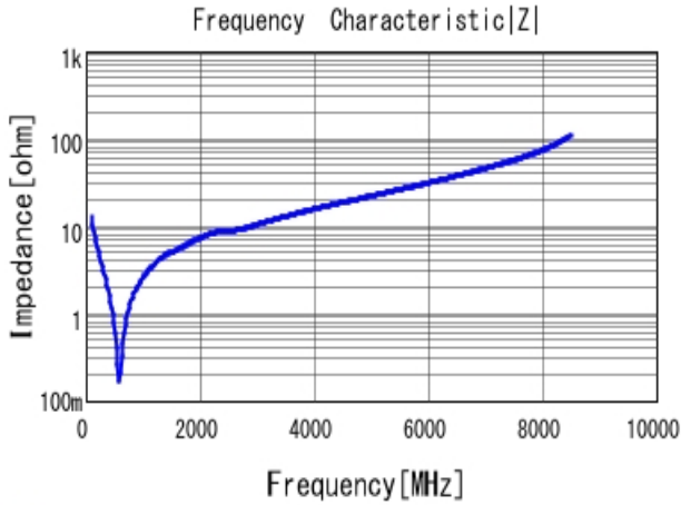
■ GRM1885C2A121JA01 |Z| DCOV, 25degC
