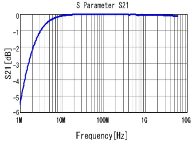
■ GRM1885C2A102JA01 S21 DCOV, 25degC
