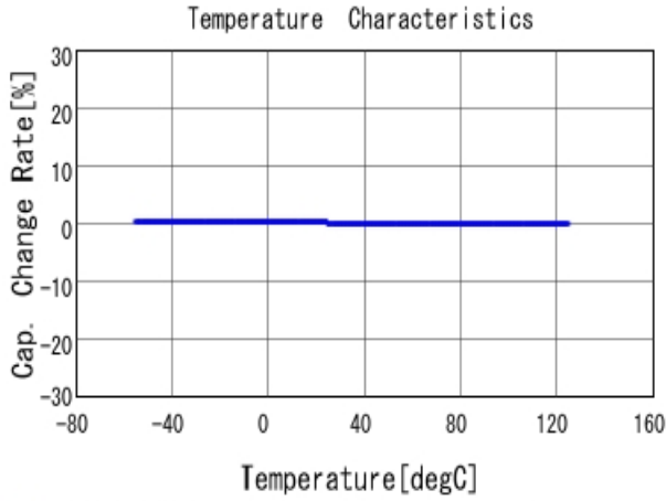
■ GRM1885C2A102JA01 C-Temp. capchange, DCOV, AC1Vrms
