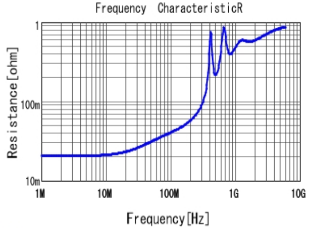
■ GRM1885C2A102JA01 R DCOV, 25degC
