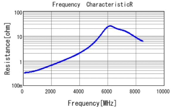
■ GRM1885C2A100JA01 R DCOV, 25degC
