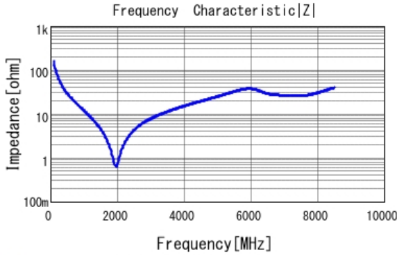
■ GRM1885C2A100JA01 |Z| DCOV, 25degC
