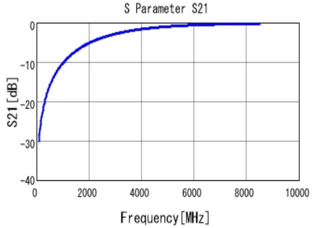
■ GRM1885C1HR50BA01 S21 DCOV, 25degC
