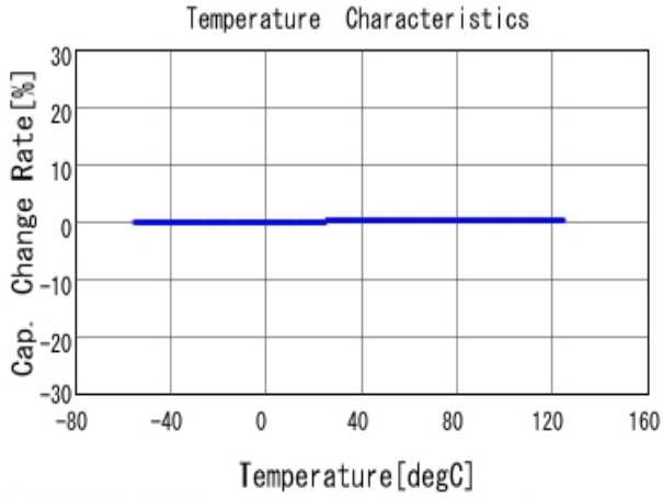
■ GRM1885C1HR50BA01 C-Temp. capchange, DCOV, AC1Vrms
