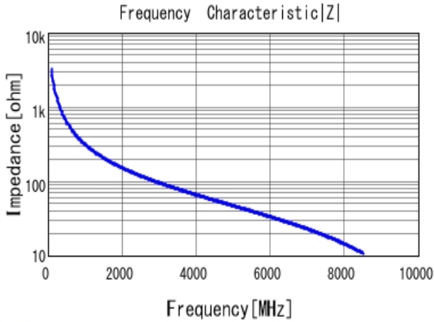
■ GRM1885C1HR50BA01 |Z| DC0V, 25degC
