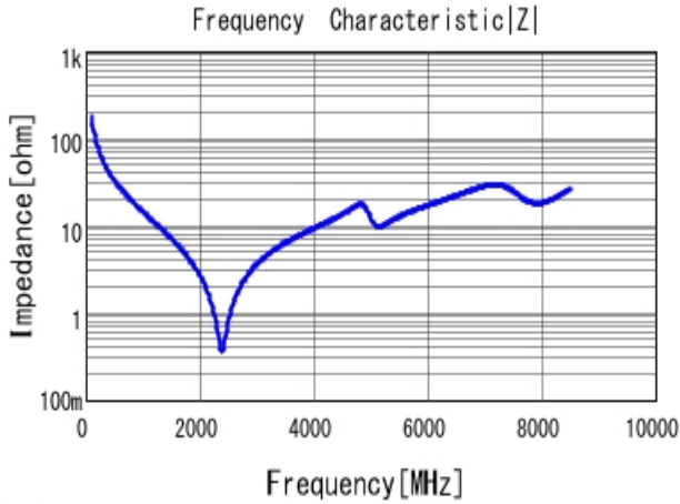
■ GRM1885C1H9R1DA01 |Z| DCOV, 25degC
