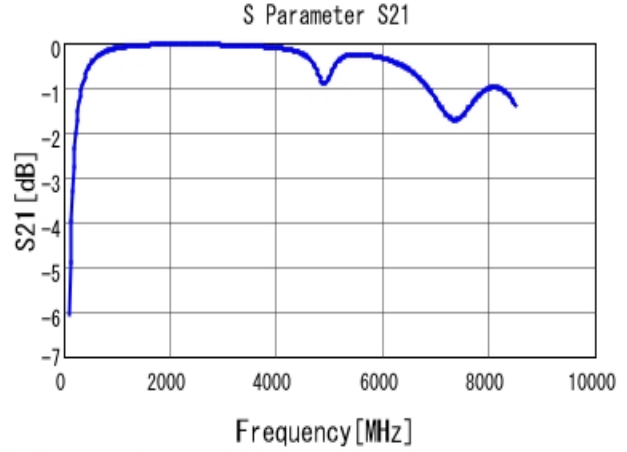
■ GRM1885C1H9R1DA01 S21 DCOV, 25degC
