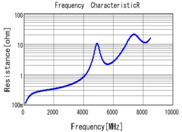
■ GRM1885C1H9R1DA01 R DCOV, 25degC
