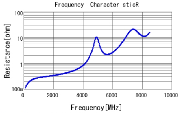
GRM1885C1H9R0DA01 R DCOV, 25degC
