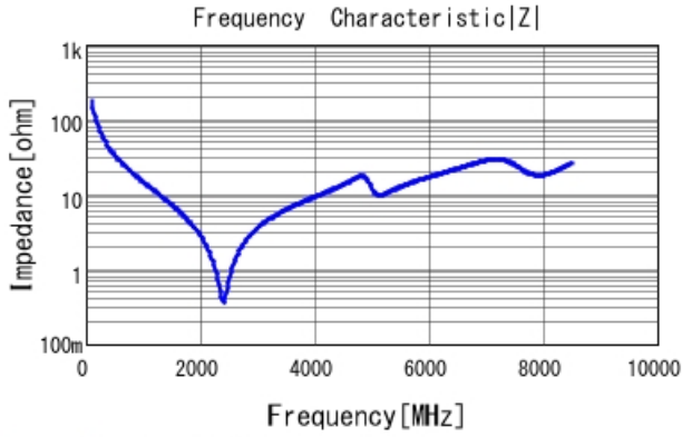
GRM1885C1H9R0DA01 |Z| DCOV, 25degC
