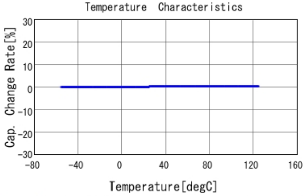
GRM1885C1H9R0DA01 C-Temp. capchange, DCOV, AC1Vrms
