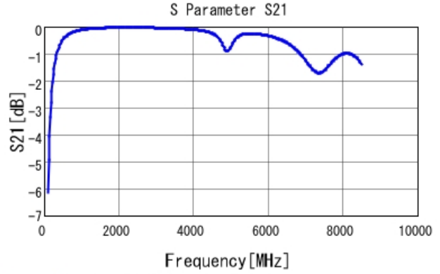
GRM1885C1H9R0DA01 S21 DCOV, 25degC
